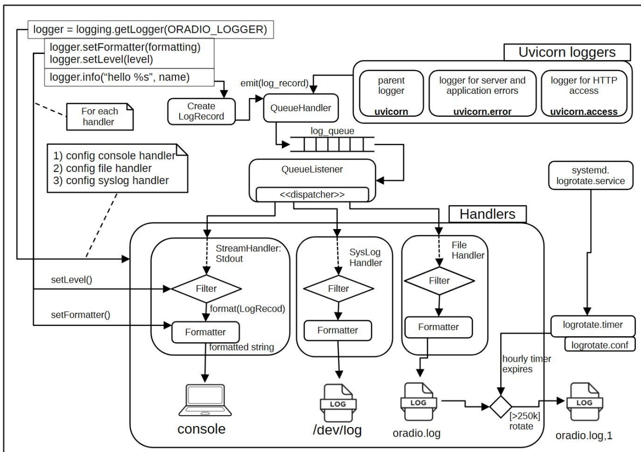
Figure 1: Logging activity diagram
