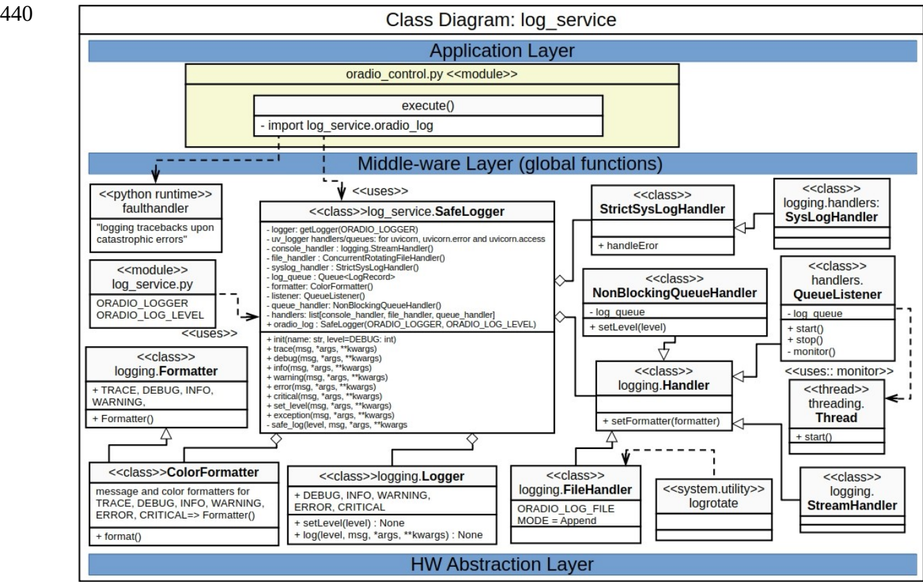
Figure 2: log_service class diagram
